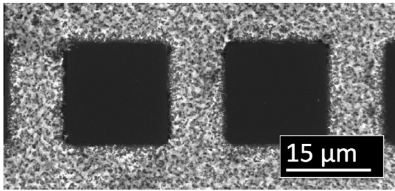
Fig. 2. SEM images gold black pattern over-coated with 150 nm SiO 2 on Si substrate. The smallest patterned feature is less than 10 μm.
