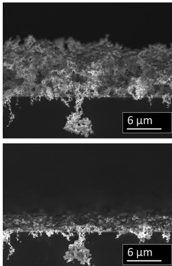
Fig. 7. Oxide over-coated gold black before (top) and after (bottom) wetting in acetone.
